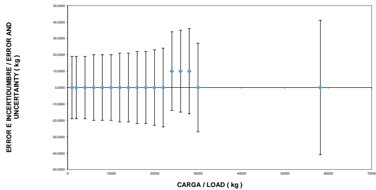
FIGURA 1. ERROR, INCERTIDUMBRE EXPANDIDA Y CARGAS / ERROR, EXPANDED UNCERTAINTY AND LOADS
